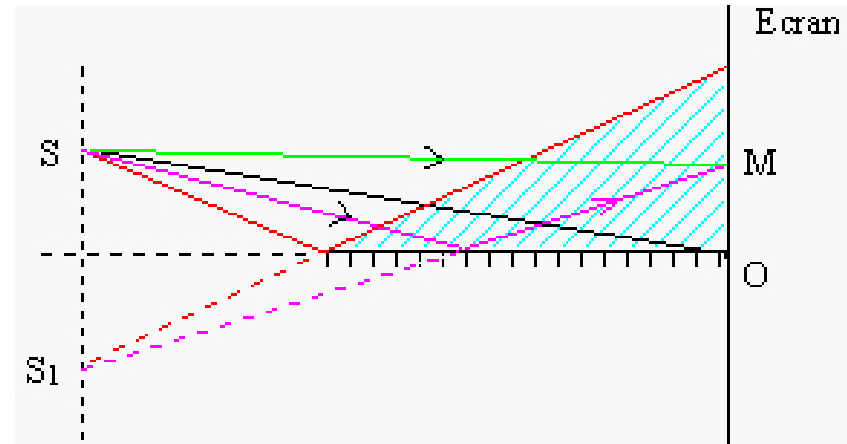
FIGURE 2 – Miroir de Lloyd
