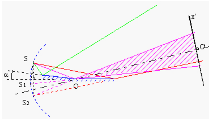
FIGURE 3 – Miroirs de Fresnel
