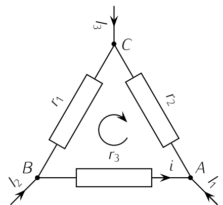
Association triangle
