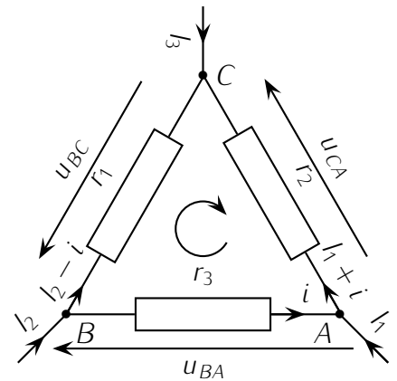
Association triangle
